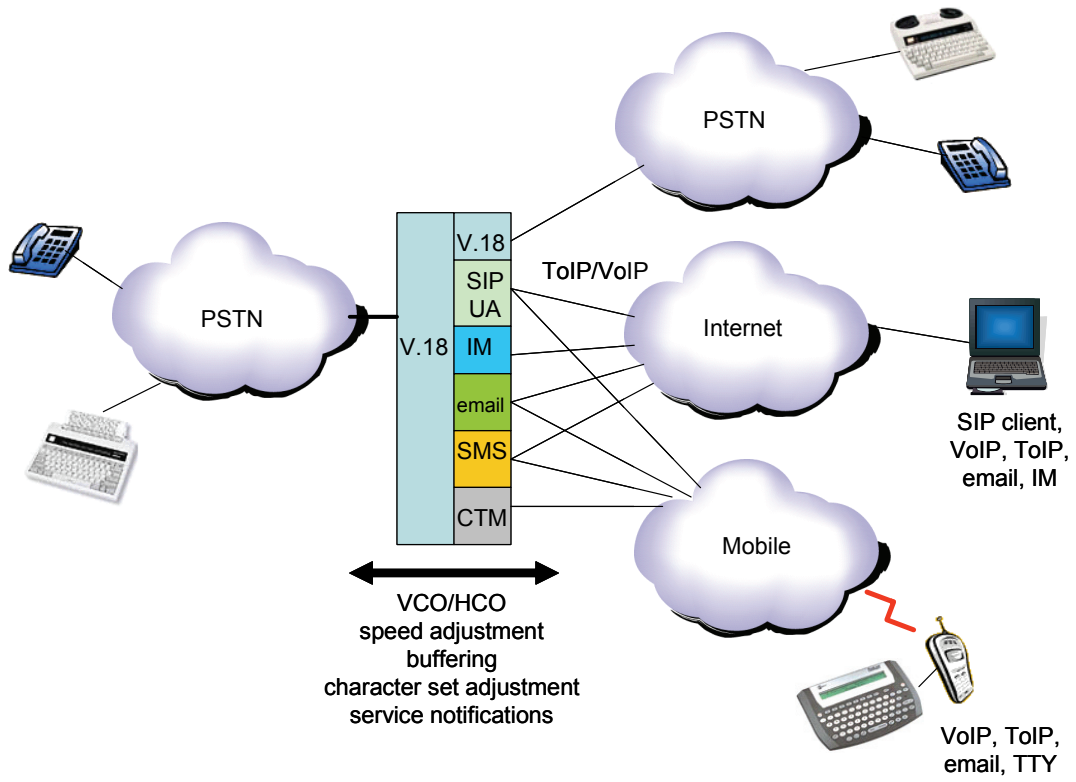
Exhibit 7.3: Possible ACIF Stage 2 server architecture [Source: Network Strategies]
