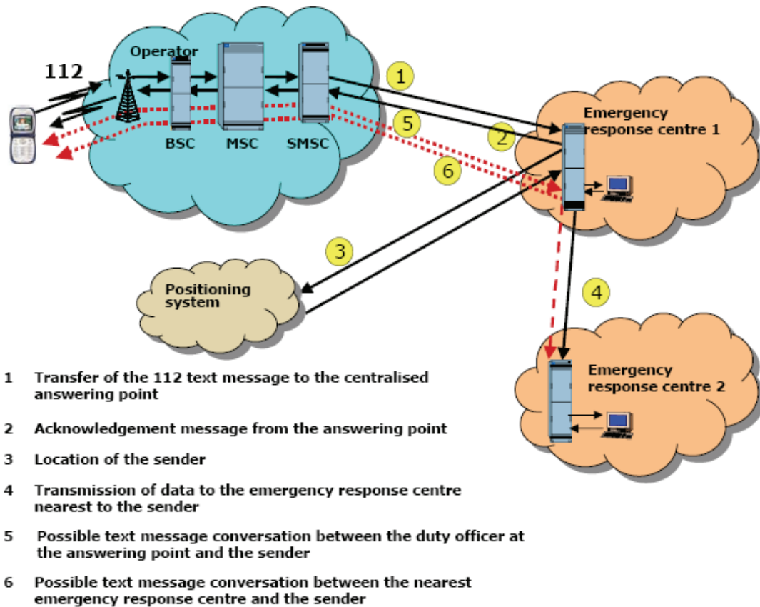
Exhibit 8.2: Implementation of the SMS emergency service [Source: FICORA Working Group for emergency communications]
