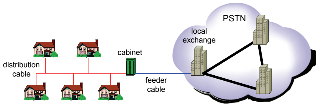
Exhibit 7.1: PSTN access network architecture [Source: Network Strategies]
